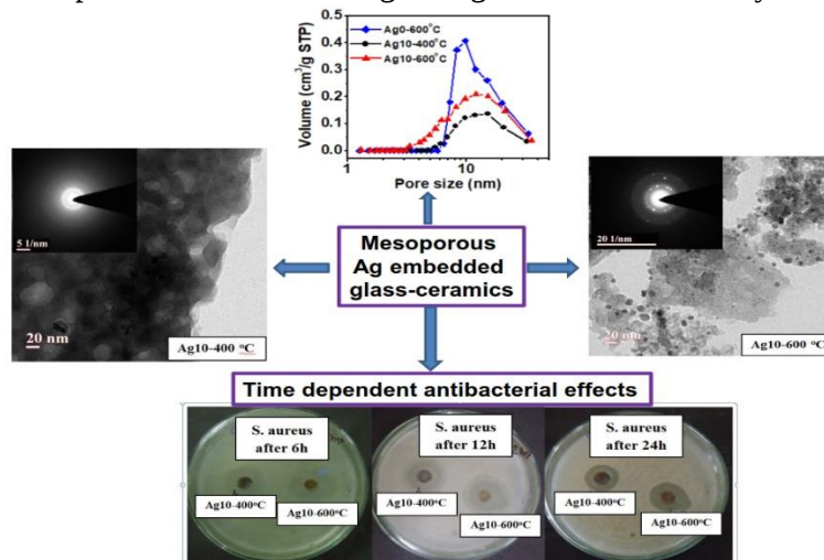
Figure 1 Ag doped calcium borosilicates 45.8 \text{ SiO}_2-(45.8-x) \text{ CaO}-8.4\text{B}_2\text{O}_3-x\text{Ag}_{20}
