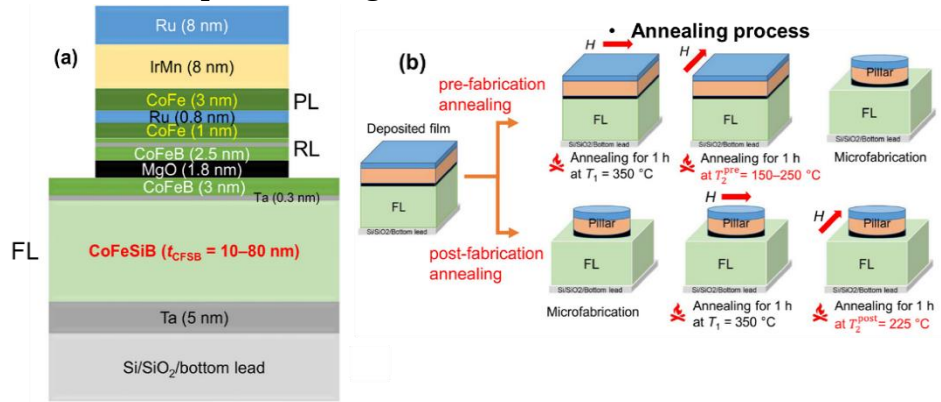
Fig.1: Schematics of (a) the layer structure of TMR sensor, (b) two different annealing process followed for the TMR sensors
