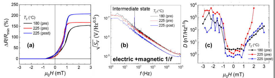
Fig.2: (a) \Delta R/R_{\text{min}} - H curves (b) noise voltage spectra for the intermediate state (at 1 mT applied field) (c) detectivity ( D ) at f = 10\text{ Hz}
